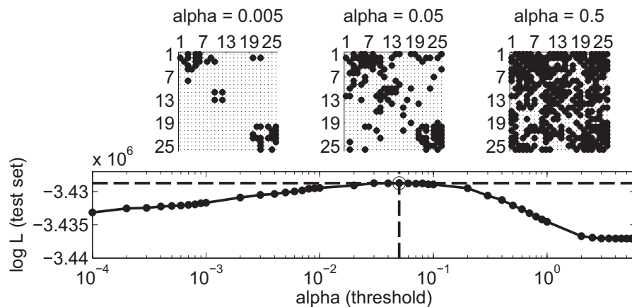
FIGURE 5 | Choice of threshold for binary connectivity matrix. The model is fitted on 80% of the data set (training set). Reduced models are created by applying a threshold \alpha on the significance value of estimated coefficients for the cross-coupling terms. The performance of the models is evaluated on the 20% remaining data (test set). Performance is measured with the log-likelihood of the data (larger value indicates a better model). A broad regime from 0.02 \leq \alpha \leq 0.08
