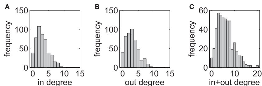
FIGURE 6 | Degree distributions, summed over all 17 data sets. (A) In-degree. (B) Out-degree. (C) Summed in- and out-degrees per vertex. There is no indication of a power-law for any of the three distributions as it would be required for scale-free networks.
