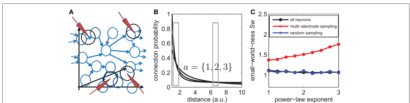
FIGURE 10 | Localized sub-sampling overestimates true small-world-ness. (A) Scheme of the simulation of the network topology. Neurons were placed in a 3D volume and linked with a distance-dependent wiring probability. Virtual electrodes were placed in the volume assuming that each electrode can pick up the neurons and their connections within a certain radius around the electrode tip. This represents the typical sampling geometry of multi-electrode recordings. (B) The distance-dependent probability was assumed to be a power-law with a constant baseline p(d) = p_0 + kd^{-a} . The simulations were repeated for different exponents a . The distributions are shown here for a = 1, 2, 3 . The
